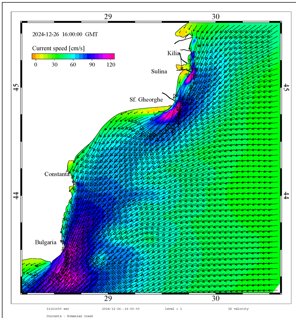
Fig. 10. Surface currents modelling (SHYFEM).
