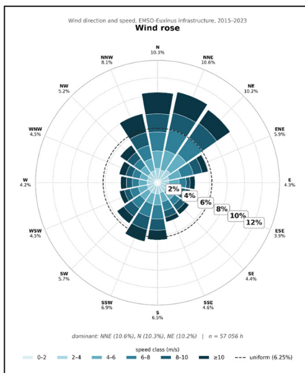
Fig. 7. Wind predominant parameters between years 2015–2023.
