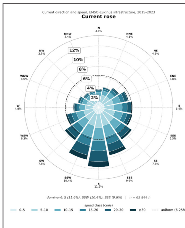
Fig. 8. Current predominant parameters between years 2015–2023.
