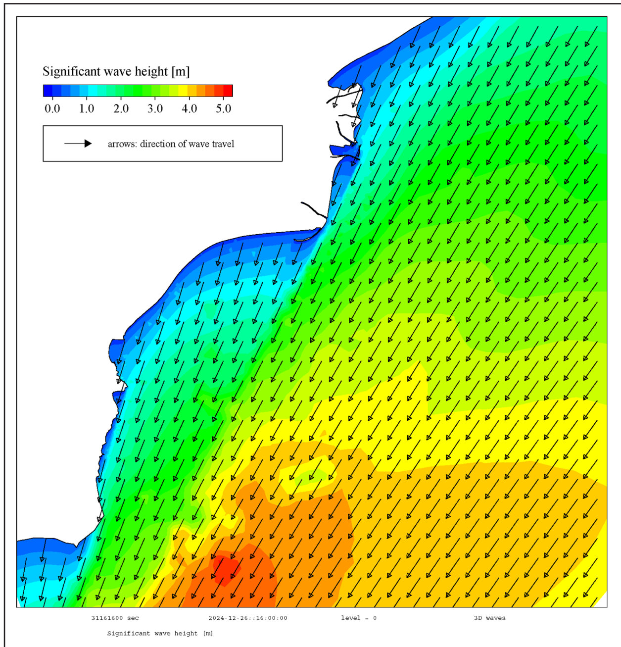
Fig. 9. Significant wave height modelling (SHYFEM).
