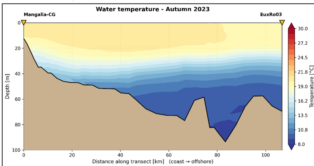
Fig. 5. Water temperature – Autumn 2023 – Mangalia transect CC-EuxRo03.
