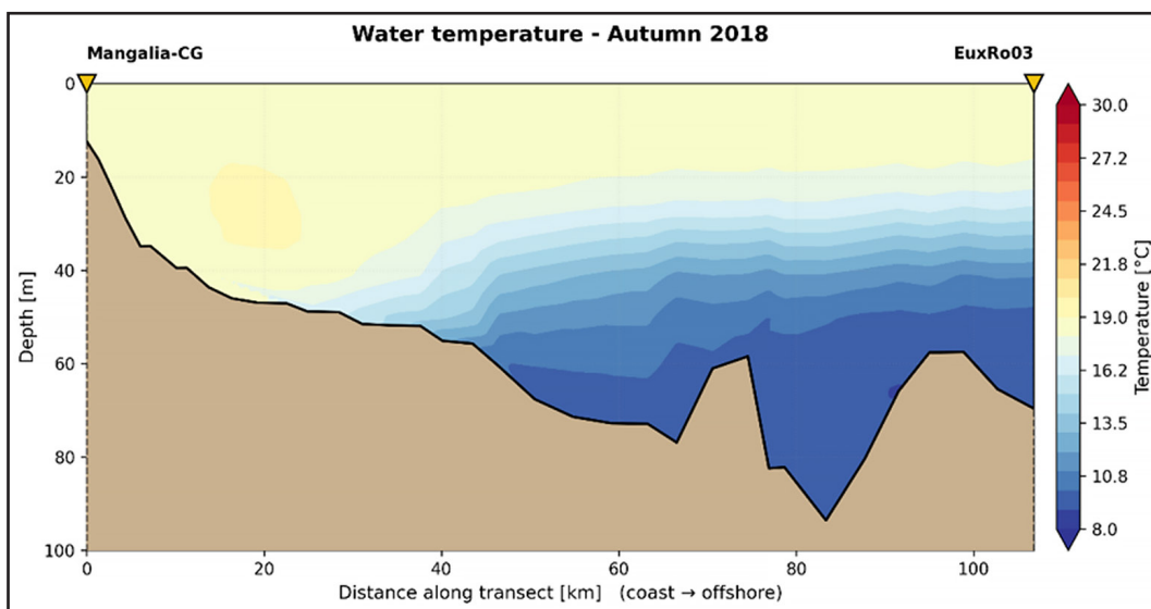
Fig. 4. Water temperature – Autumn 2018 – Mangalia transect CC-EuxRo03.
