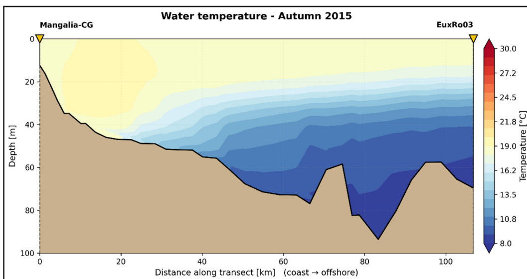
Fig. 3. Water temperature – Autumn 2015 – Mangalia transect CC-EuxRo03.
