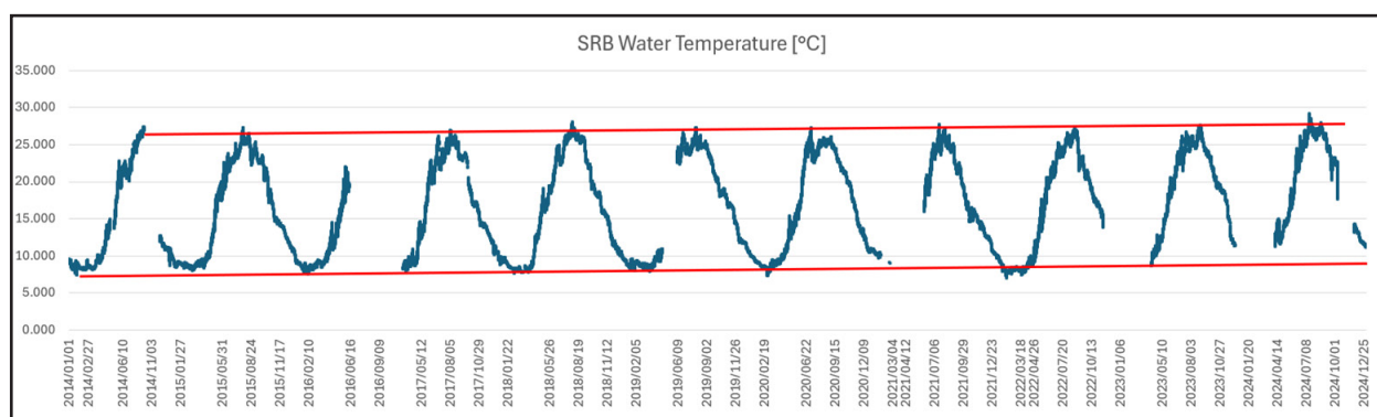
Fig. 2. Water temperature evolution between years 2014–2024.
