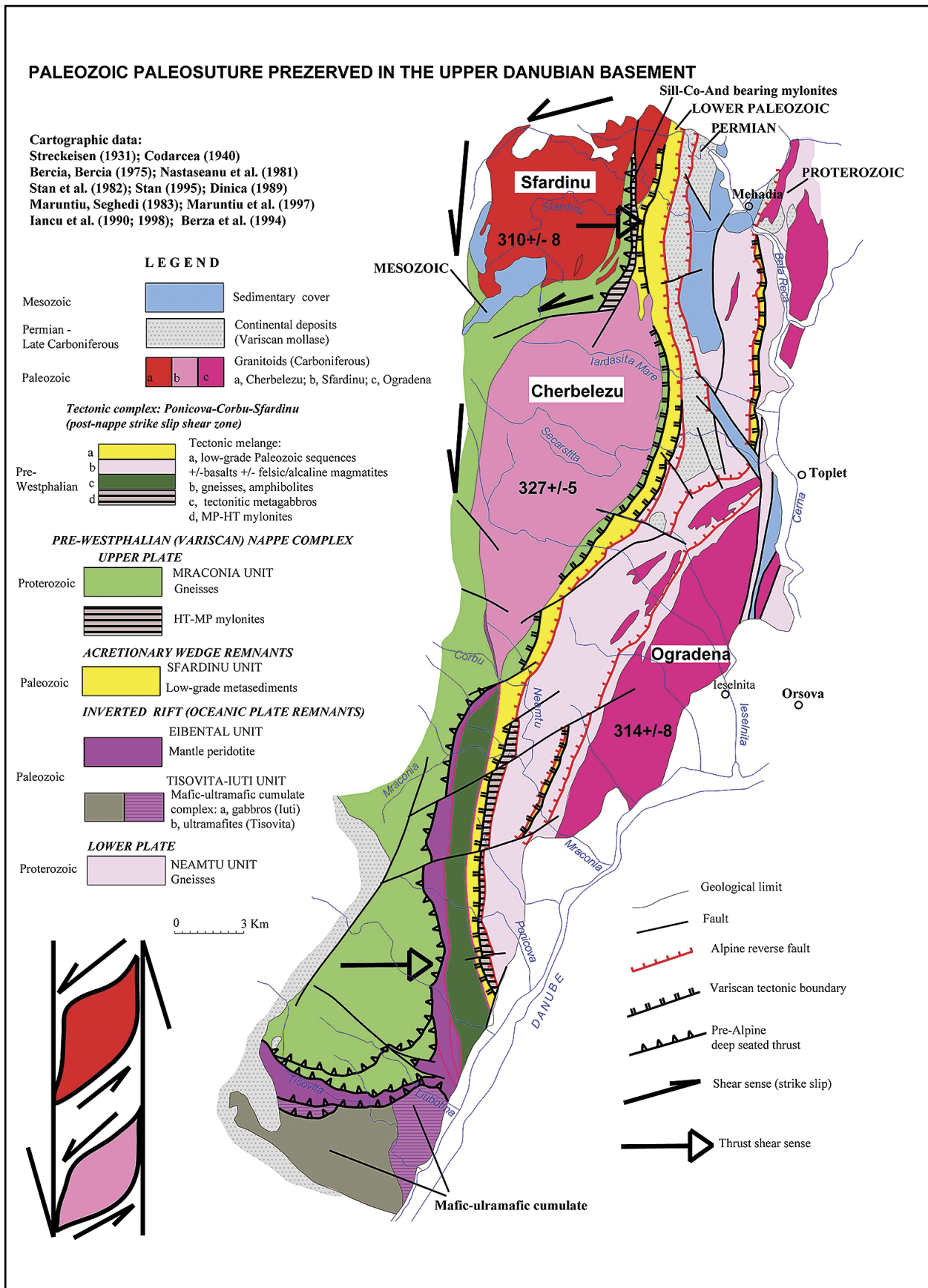
Fig. 4. Neoproterozoic – Lower Paleozoic basement in the South Carpathians and Variscan imprint. Abbreviations as in Fig. 3
