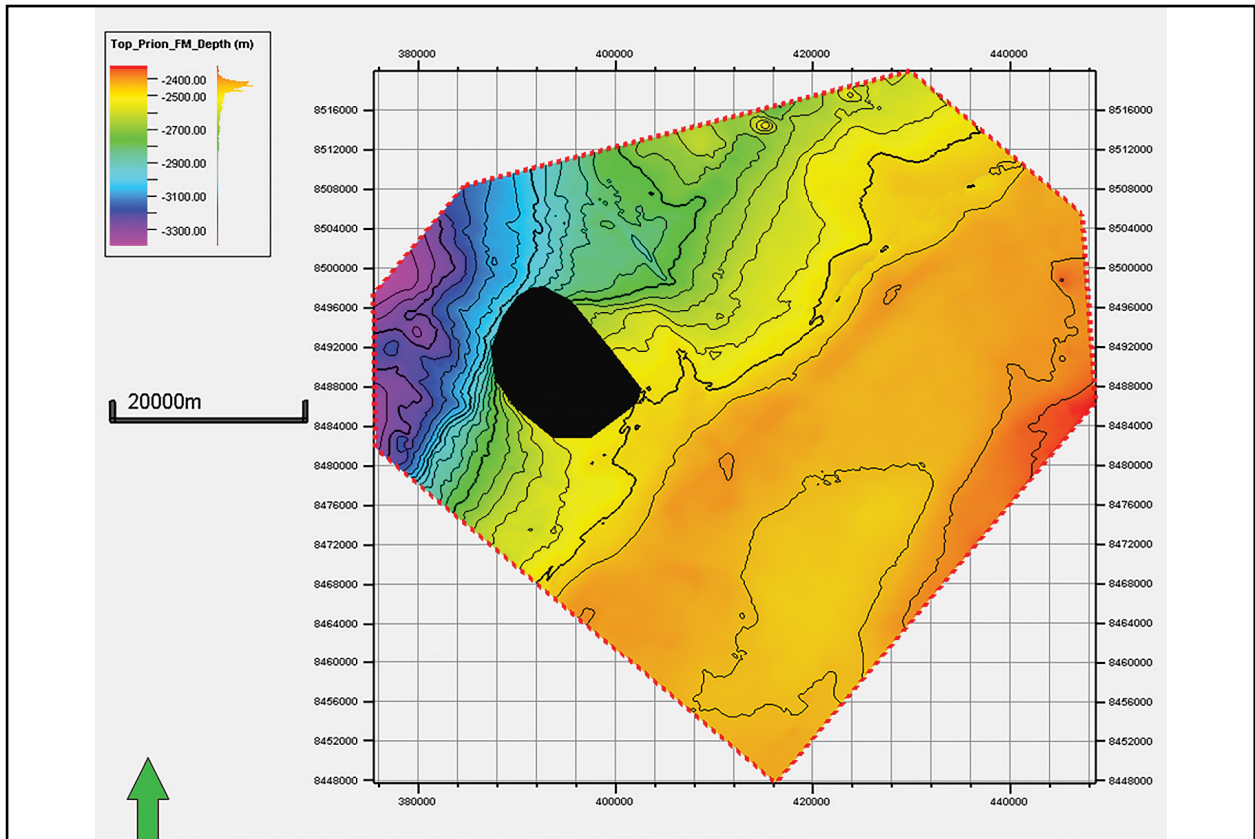
Fig. 5. Structural depth map for the top of the Prion Fm. It reflects that the succession deepens toward the North-West.
