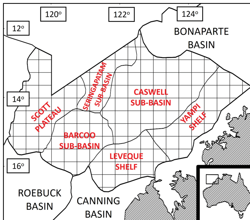
Fig. 1. Location and distribution of the Browse Basin along with the main tectono-stratigraphic units and the surrounding basins (after Rollet et al. , 2016).
