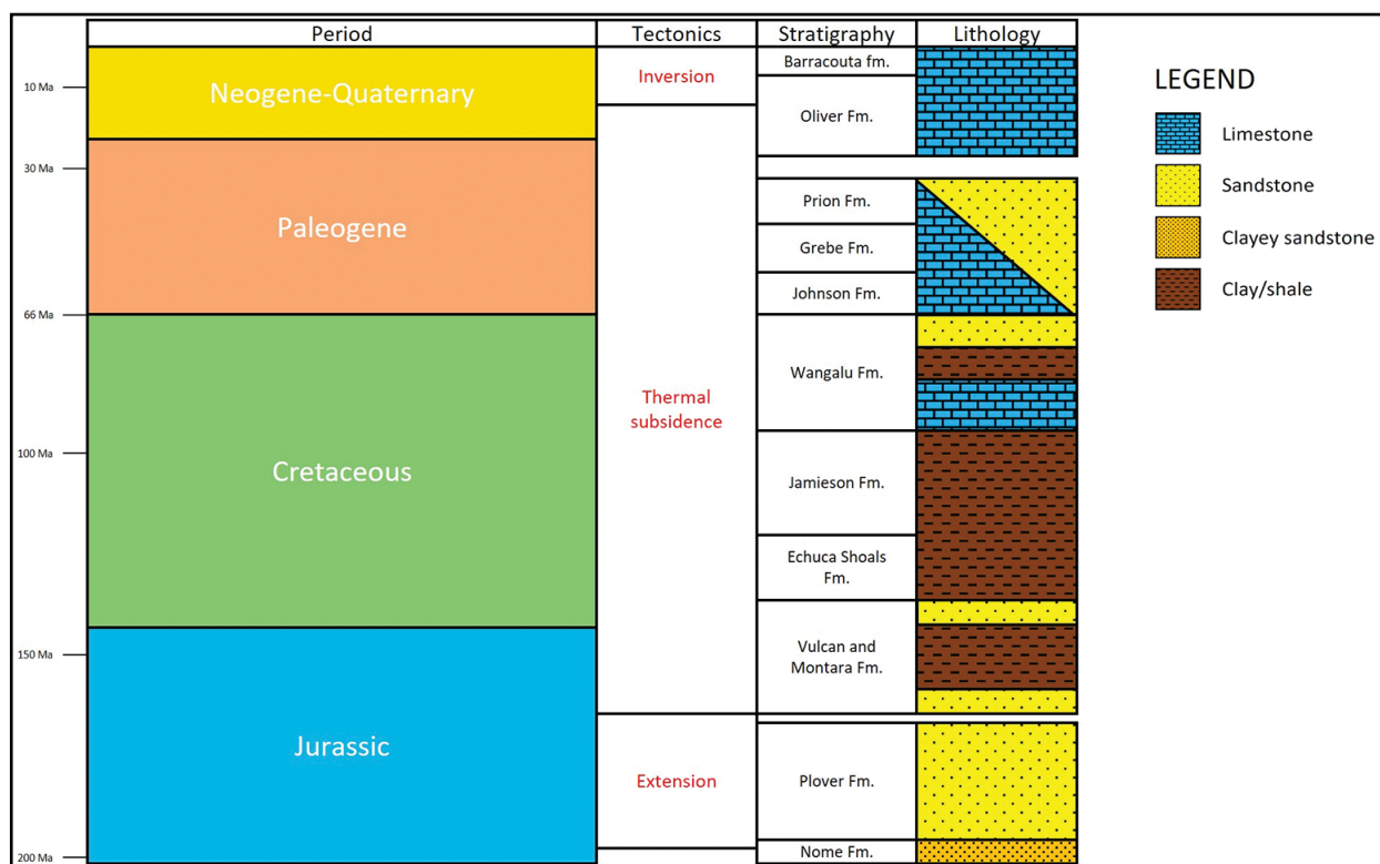
Fig. 2. Tectono-stratigraphic chart for the Browse Basin (Caswell sub-basin) (after Geoscience Australia, 2022).
