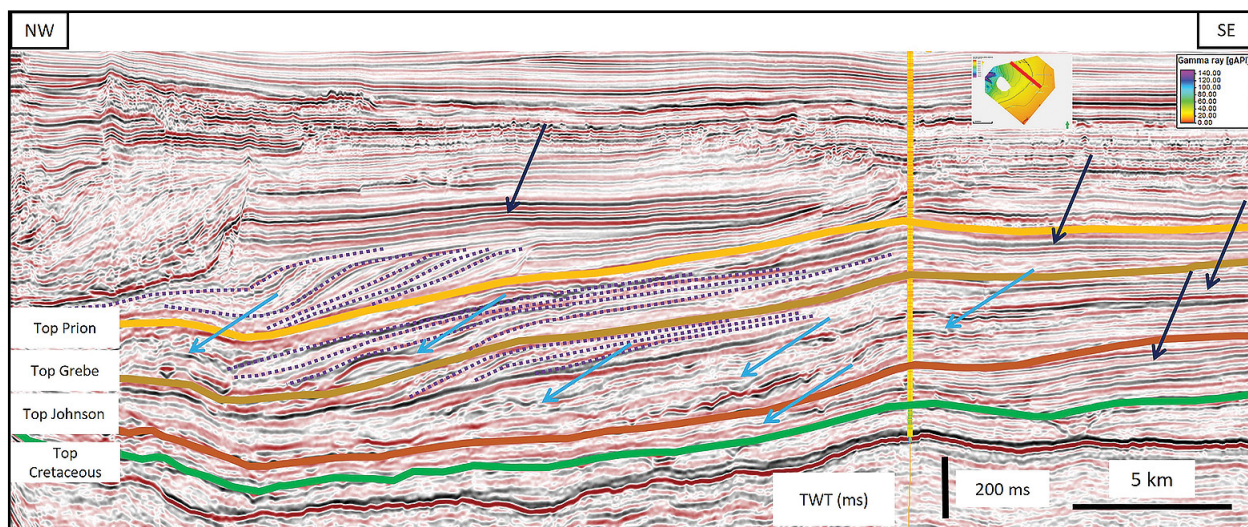
Fig. 7. Seismic profile (TWT) showing the Paleogene prograding systems (dotted purple lines) and the typical facies for shelf environments (parallel reflectors – dark blue arrows) and submarine fans (chaotic reflectors – light blue arrows).
