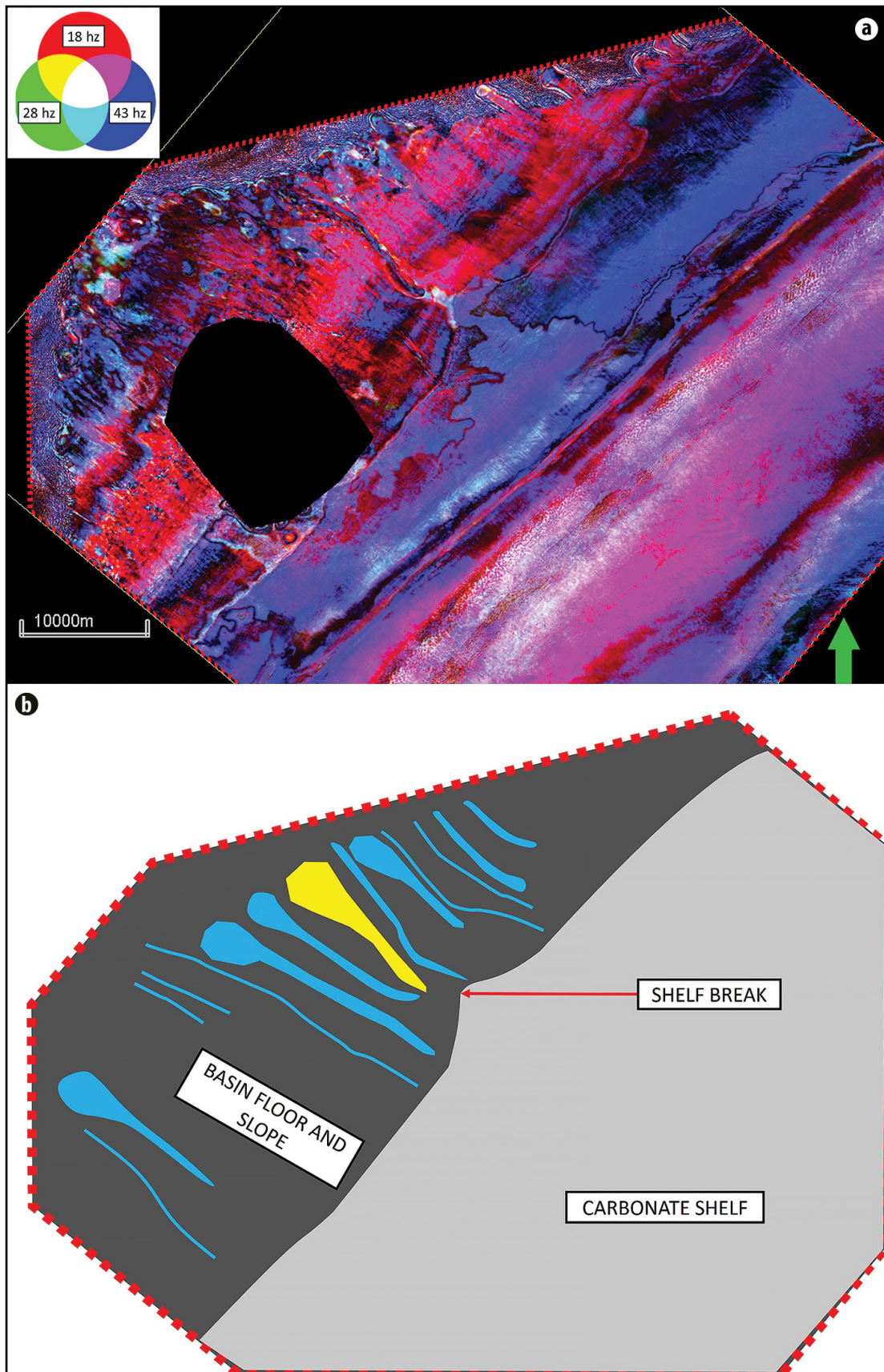
Fig. 8. Time slice at -2488 ms from the GSD volume flattened at the top of the Prion Fm. (a) that was used to build the stratigraphic model for the sedimentological evolution of the Prion Fm. in the deep water environments. (b) The yellow submarine fan system represents the Prometheus prospect.
