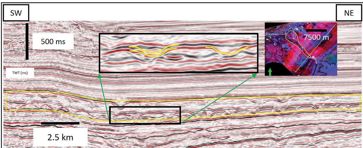
Fig. 10. Seismic profile revealing the channel-levee systems that are included in the submarine fans.
