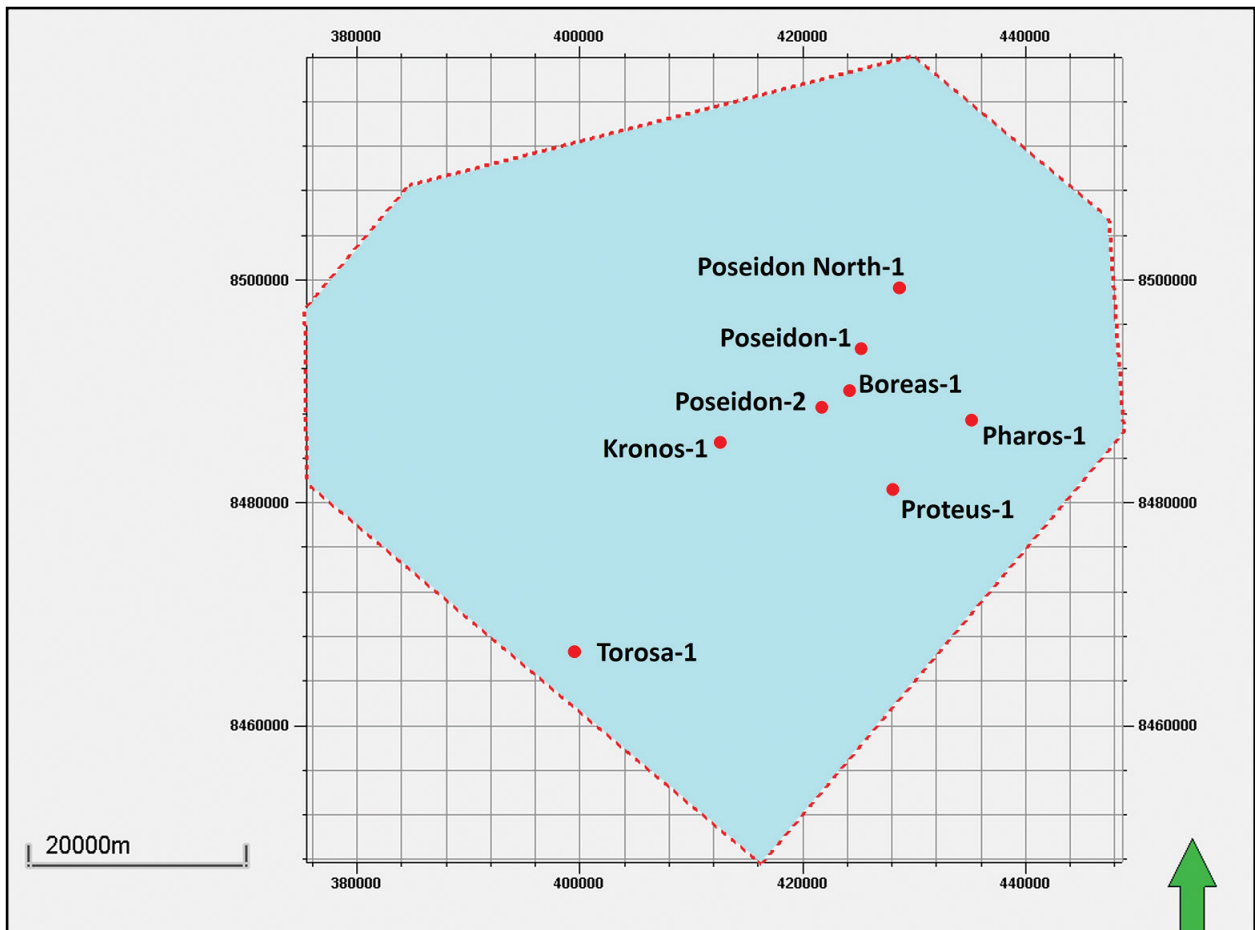
Fig. 3. Location of the Poseidon 3D seismic survey and the position of the available wells that were used in this project.
