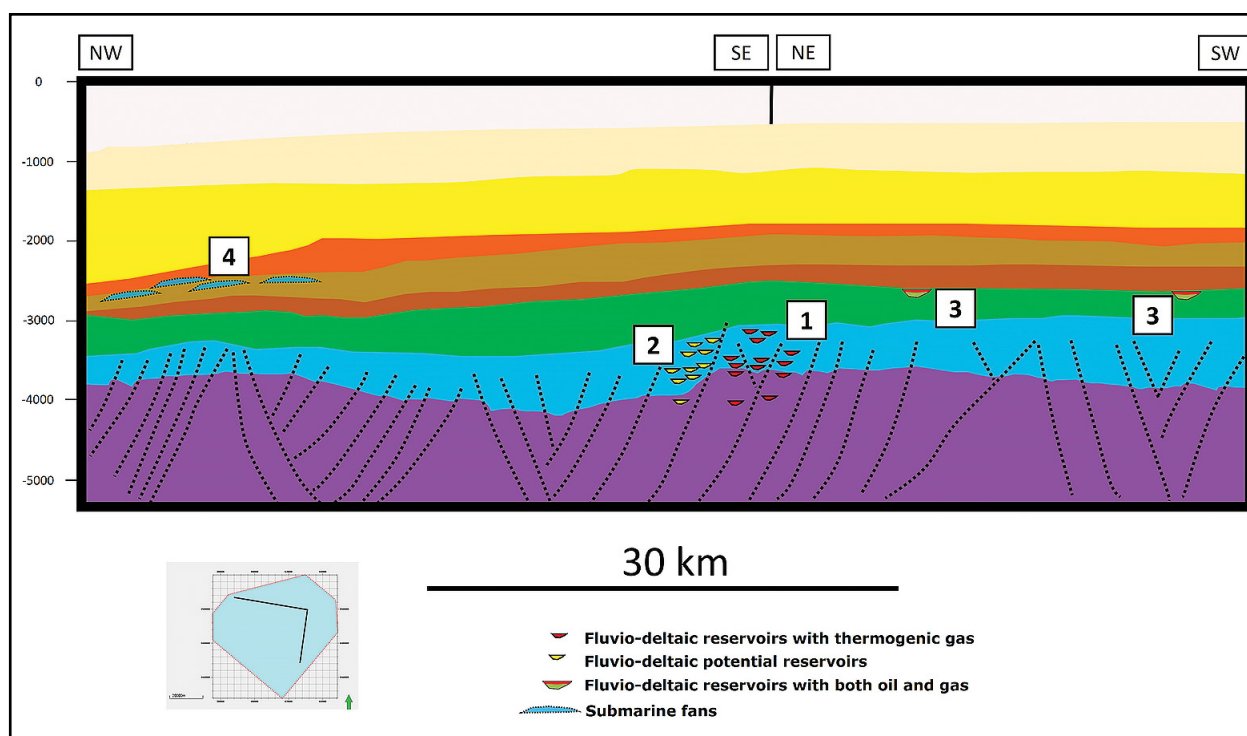
Fig. 4. Regional TWT (ms) cross section along the study area showing the stratigraphy and the main petroleum plays that were identified: 1) Plays with anticline structures and tilted blocks that include Triassic and Jurassic fluvio-deltaic reservoirs with thermogenic gas (proven play throughout the Browse Basin in the syn-rift Plover Fm., including the Poseidon field that is located in the study area); 2) Plays with monocline structures that include Triassic and Jurassic fluvio-deltaic reservoirs with thermogenic gas (an extension to the north of the play that defines the Poseidon field); 3) Plays with stratigraphic traps (and minor structural element) in upper Cretaceous oil and gas-bearing deltaic reservoirs (there have been several discoveries in upper Cretaceous reservoirs from the Browse basin); 4) Plays with stratigraphic traps in upper Eocene-lower Oligocene oil and gas-bearing turbidite reservoirs (not proven yet).
