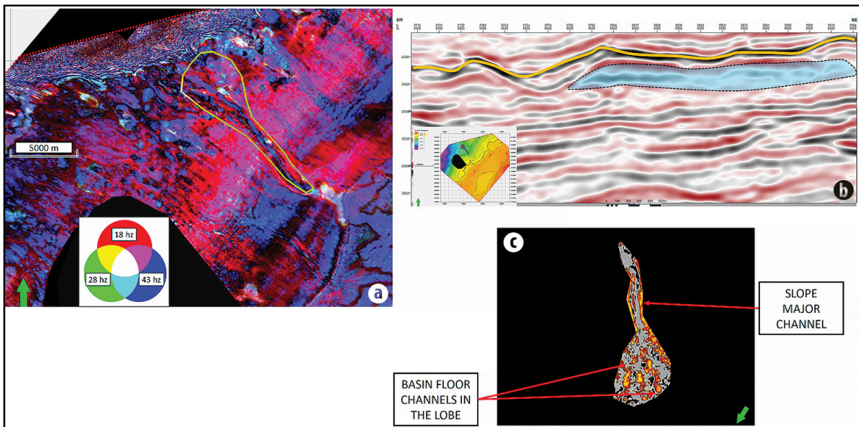
Fig. 9. A closer look at the GSD time slice that was used to delineate the submarine fan system of the Prometheus prospect, (a) along with a seismic section where the specific lobe morphology was identified (the position of the profile is figured on the map). (b) The RMS Amplitude volume shows specific morfosedimentary features of the turbidite: (c) slope major feeder channel and basin floor lobe channels.
