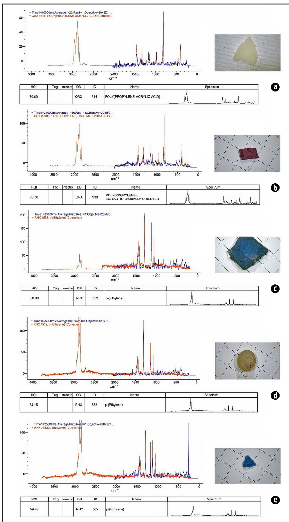
Fig. 4. Examples of Raman microspectrometry results: (a, b) Polypropylene; (c, d, e) Polyethylene; the x axis represents the wavenumber ( \text{cm}^{-1} ) and the y axis represents the intensity of the scattered light.
