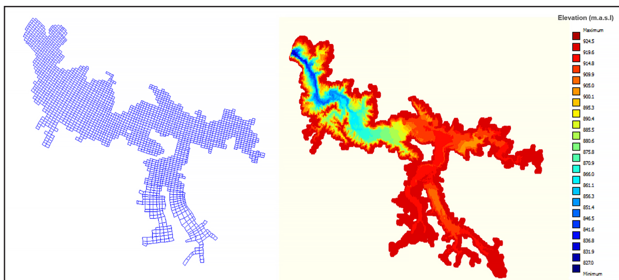
Fig. 2. Grid (left) and elevation (right) of Porce II reservoir.
