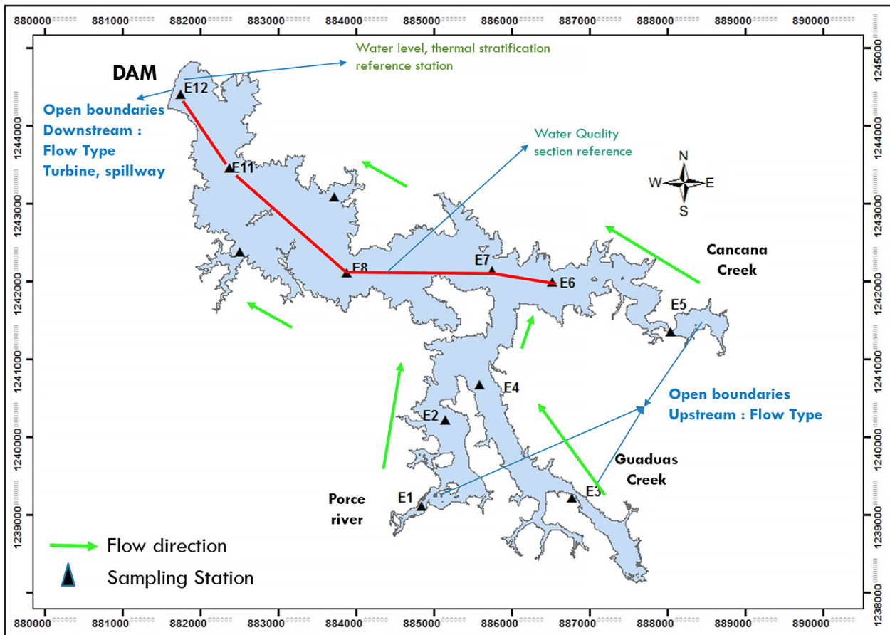
Fig. 3. Porce II model extent and water quality sampling stations location.
