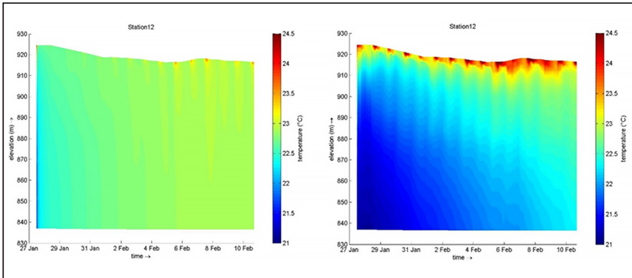
Fig. 5. Temperature profile in station 12 before and after the calibration process.
