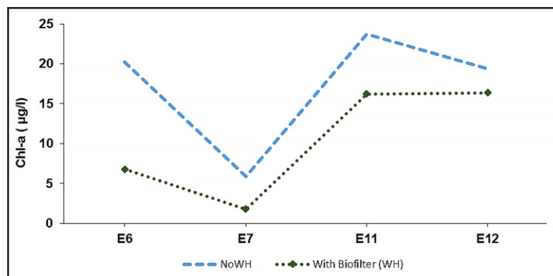
Fig. 7. Simulated chlorophyll-a concentration in a transect of Porce II reservoir with and without presence of Water Hyacinth (WH).
