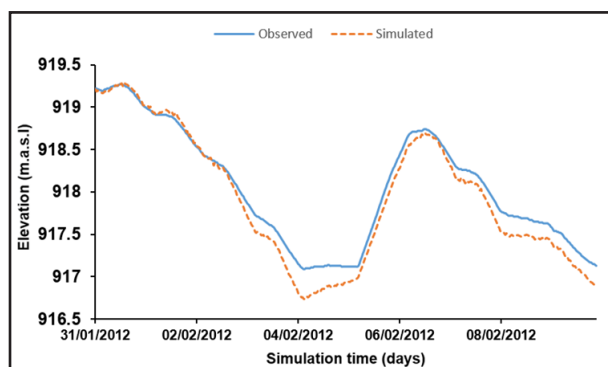
Fig. 4. Water level Porce II reservoir.
