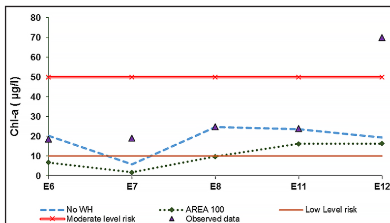
Fig. 9. Critical chlorophyll-a concentration for health risk in Porce II reservoir.
