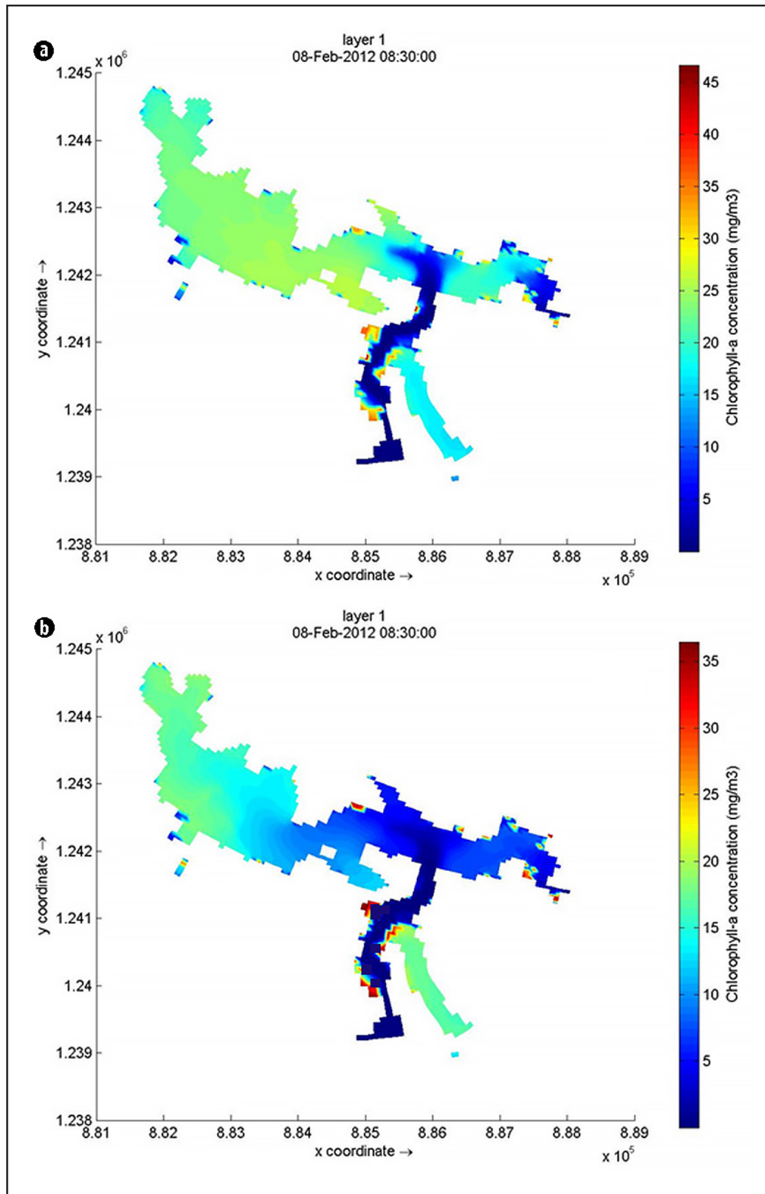
Fig. 8. Effect on chlorophyll-a with biofilter using Water Hyacinth (a) without macrophytes (b) biofilter of an area of 100 hectares.
