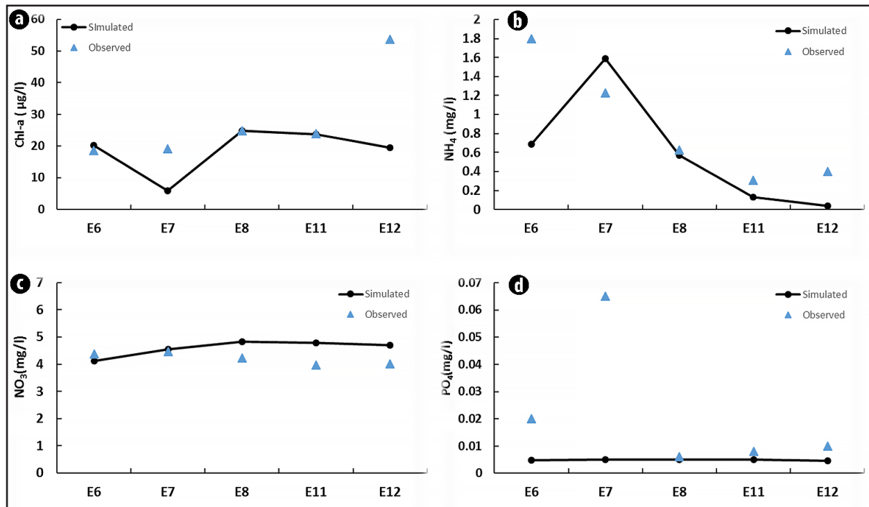
Fig. 6. Observed and simulated (a) chlorophyll-a, (b) ammonium, (c) nitrate and (d) phosphorus concentrations in a transect Porce II reservoir model. E6 and E7 are stations close to the mouth and E12 is the dam.
