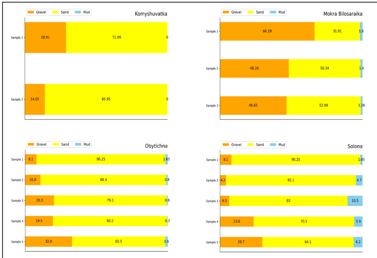
Fig. 2. Granulometric compound for each river.
