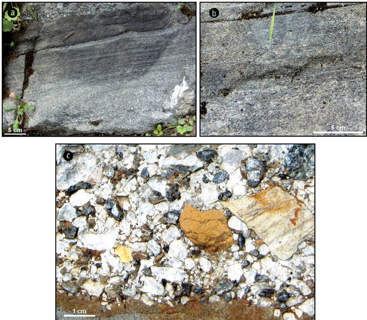
Fig. 8. Raciú Breccia with normal grading and parallel lamination. Images (b) and (c) show details from the upper and lower parts of the graded layer (a), respectively. Jepsi River, Buşteni town.
