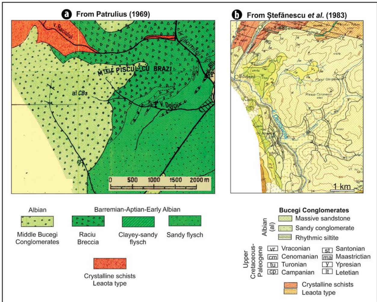
Fig. 3. Albian deposits in the Ialomița-Dâmbovița area, on Patrulius (1969) map and the geological map of Romania at 1:50,000 scale (Ștefănescu et al. , 1983).
