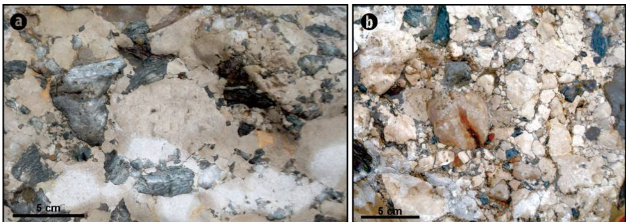
Fig. 9. Matrix in Raciú Breccia. (a) Raciú Breccia without matrix, with interlocked limestone clasts. (b) Raciú Breccia with matrix. Ialomiţa River, downstream from the confluence with Gâlmei River.
