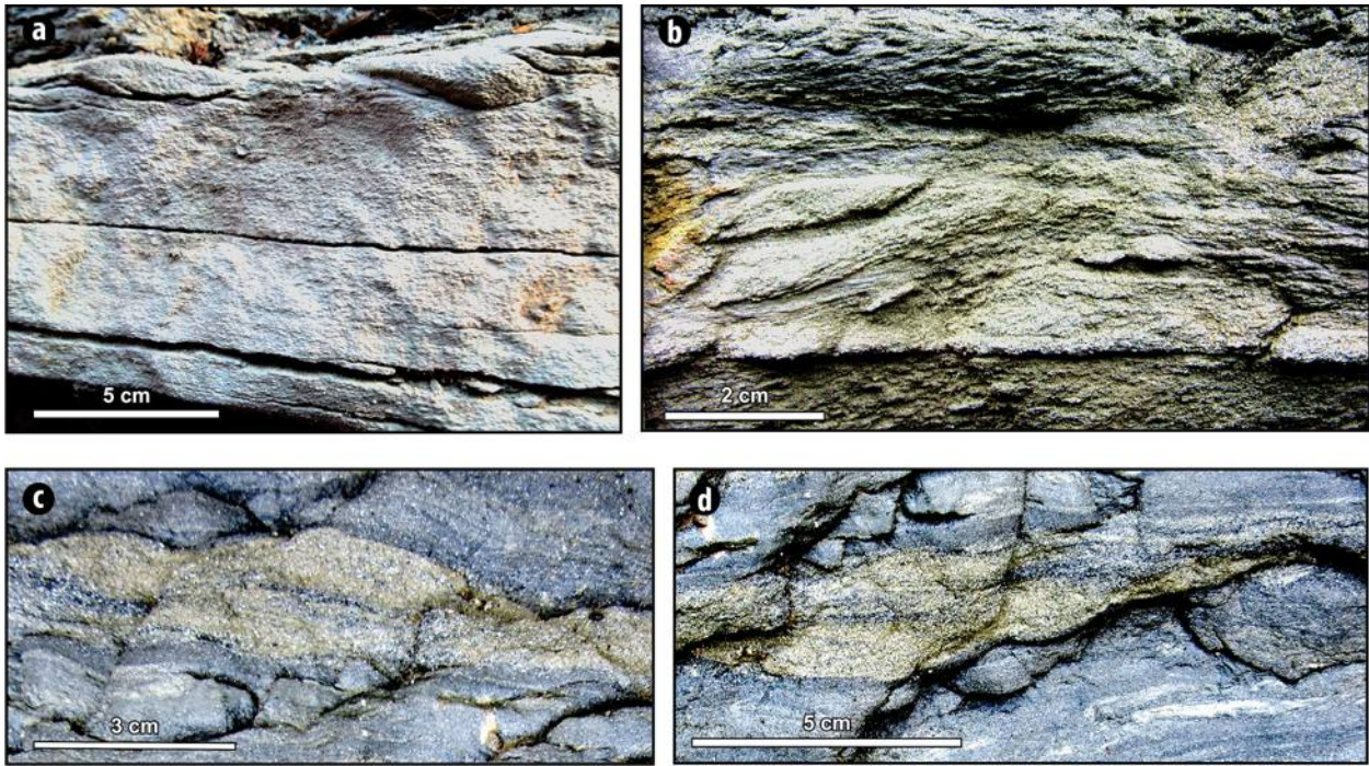
▲ Fig. 30. Current ripples in silty and fine-grained sandstones. Comments in text. Runcu River. The ripples at the top of the sandstone bed are clearly visible (a). Two centimetres thick current ripple set in image (b) Complex cross-lamination developed in the silty lens-like bodies – (c) and (d).
