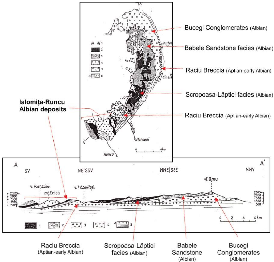
Fig. 37. Large-scale progradation of the Bucegi Mountain Albian deposits. Annotated, original figures from Jipa (1982). Legend: 1. Siltstones and fine-grained sandstones (Albian). 2. Medium- and coarse-grained sandstones (Albian). 3. Sandstone-conglomerates (Ialomița-Dâmbovița area) (Albian). 4. Bucegi Conglomerates. 5. Răciu Breccia in the Moroeni Formation (Aptian to Early Albian). The idea of the progradation relies on the overlap of the successive Albian lithostratigraphic horizons of the Bucegi Albian deposits, each of which have direct contact with the underlying Răciu Breccia.
