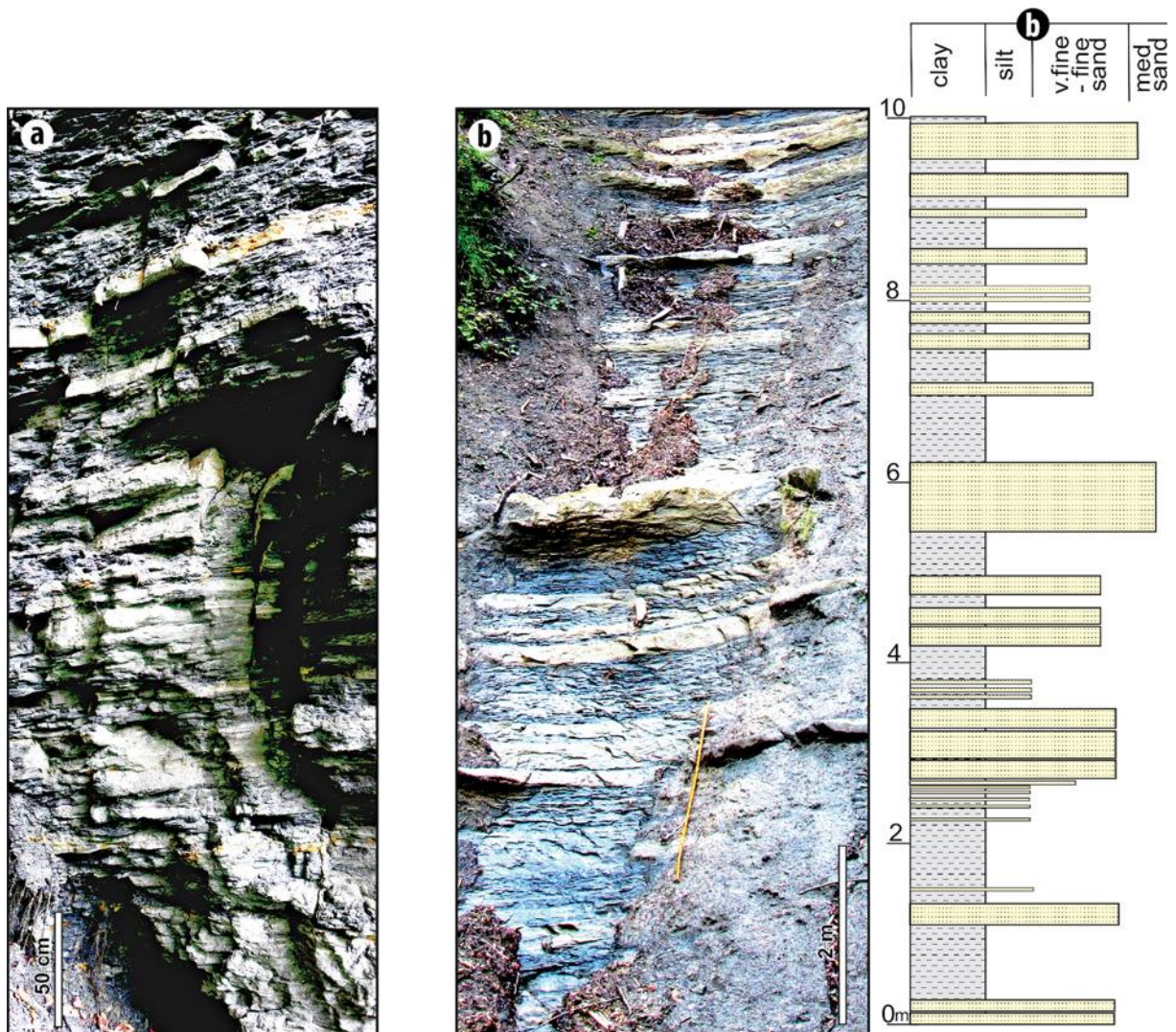
Fig. 26. Silty and fine-grained sandstone sedimentary succession. (a) Runcu River. (b) Chiliilor River, left-bank tributary. The fine-grained sandstone interbeds are more frequent in the Runcu sedimentary succession.
