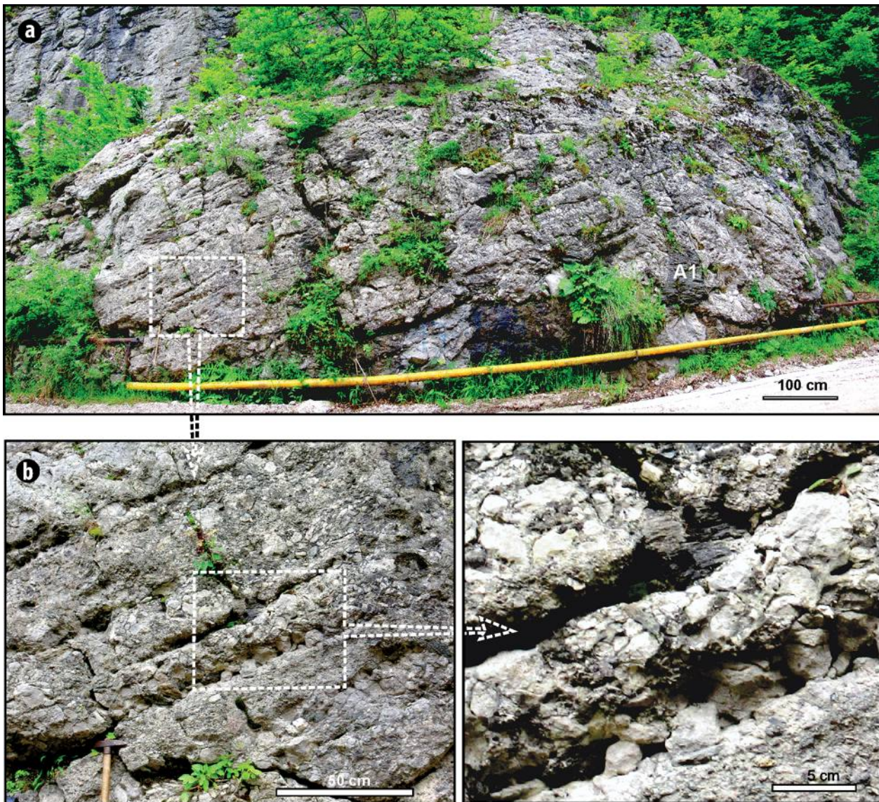
Fig. 7. Raciú Breccia from Ialomița River (upstream of the confluence with Galmei River). (a) Conglomeratic (calciudite) facies, showing an oversized metamorphic clast (A1). (b) Close up showing alternating medium- to coarse-grained and very fine-grained Raciú Breccia.
