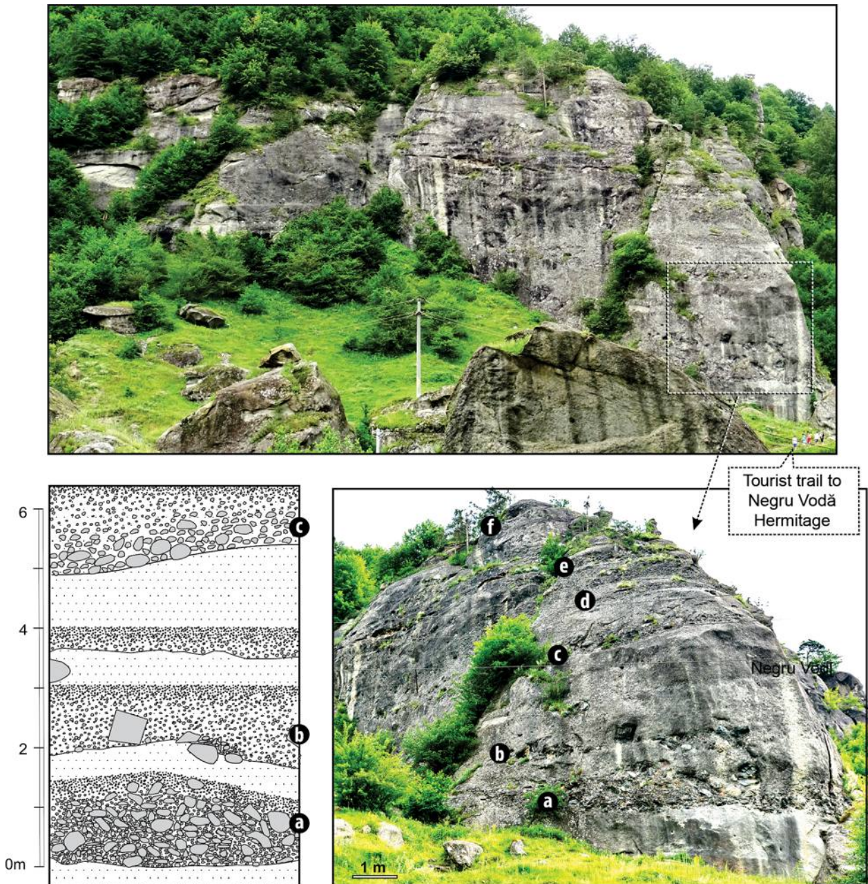
Fig. 22. Albian sandstones with intercalations of coarse- and very coarse-grained conglomerates (a) to (f). Sketch shows textural details of intercalations (a), (b) and (c). The conglomerate beds are intercalated in a prevailing sandstone succession. Outcrop on the western slope of Dâmbovița River, northern periphery of the Cetățeni locality.
