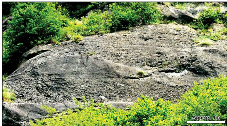
Fig. 25. Normal grading and cut-and-fill structures in the very coarse-grained conglomerate lithofacies. Outcrop on the left side of Dâmbovița valley, northern periphery of the Cetațeni locality.
