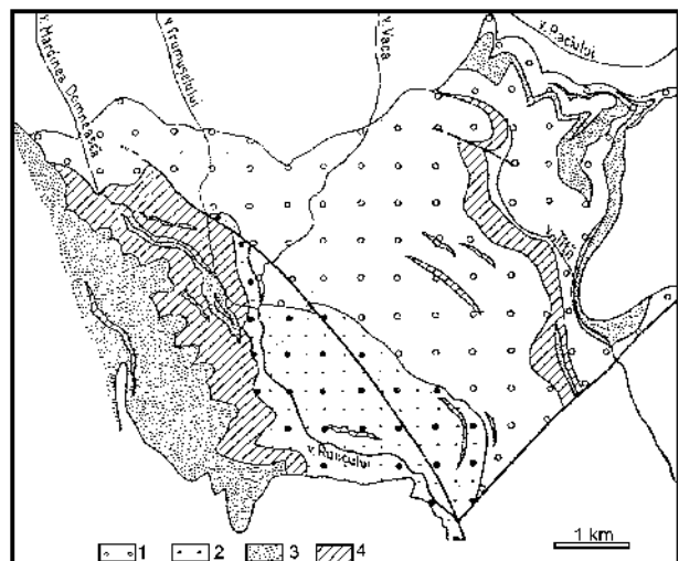
Fig. 4. Lithofacies map of the Albian deposits in the area between the Ialomița and Runcu rivers. From Jipa (1982). Legend: 1. Conglomerate. 2. Sandy conglomerate. 3. Massive sandstone. 4. Silty to fine-grained sandstones.
