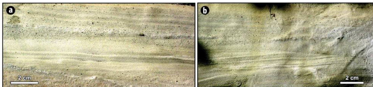
Fig. 35. Planar and low-angle cross lamination in medium-grained sandstone. The low-angle cross lamination generally occurs in relatively coarser-grained arenite sediments. Chilililor River.
