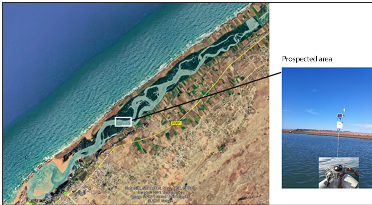
Fig. 1. ADCP and combined continuous measurement system of the Multi-Parameter Probe YSI EXO 2 and the GMX 501 weather station installation area at Park Saïdi in Oualidia.
