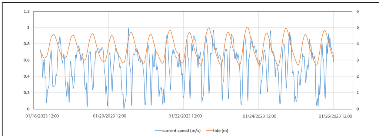
Fig. 10. Current speed recorded according to the tide measured from January 18 to 26, 2023.
