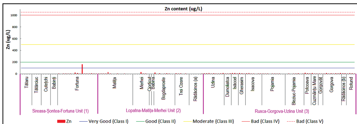
Fig. 11. Zn ( \mu\text{g/L} ) content in different samples of the investigated lakes
