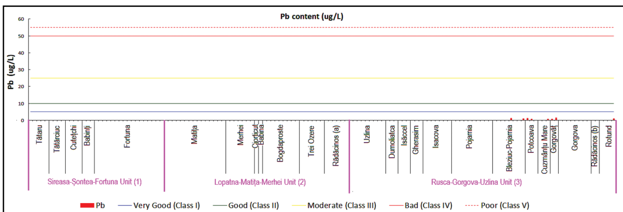
Fig. 10. Pb ( \mu\text{g/L} ) content in different samples of the investigated lakes
