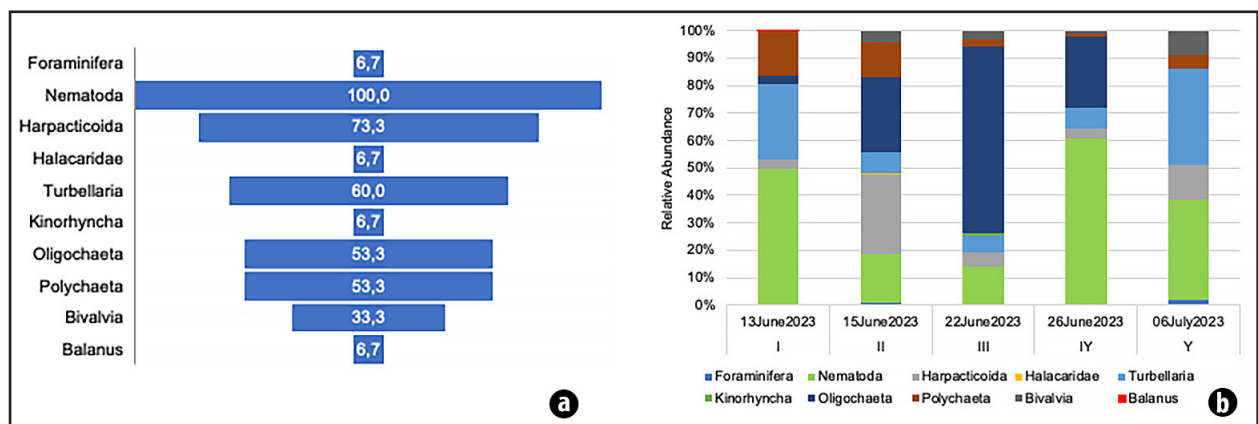
Fig. 2. Frequency of occurrence (a) and relative abundance of meiofauna taxa. Mean values of replicated samples (n = 3) are shown (b).
