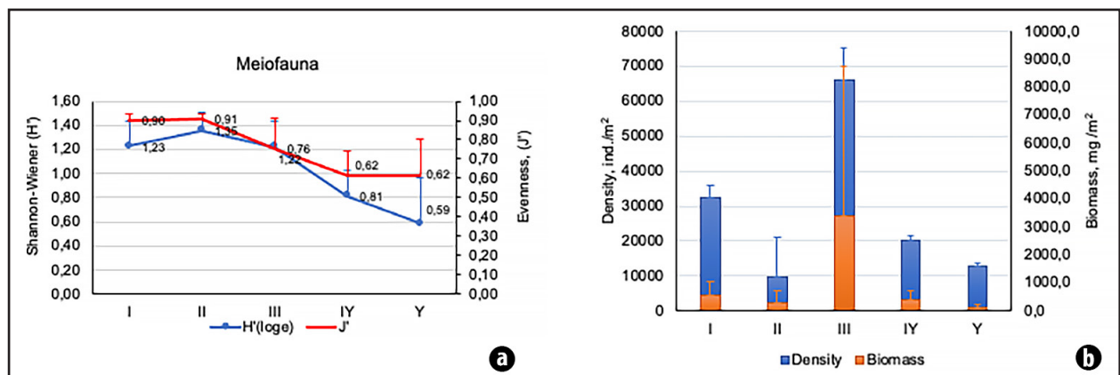
Fig. 3. Meiofaunal univariate measures. (a) Shannon-Wiener ( H' ) and Pielou's evenness ( J' ); (b) meiofauna abundance (N, ind./m 2 ) and biomass (B, mg/m 2 ) in the sublittoral zone of 0.5 m during the study periods.
