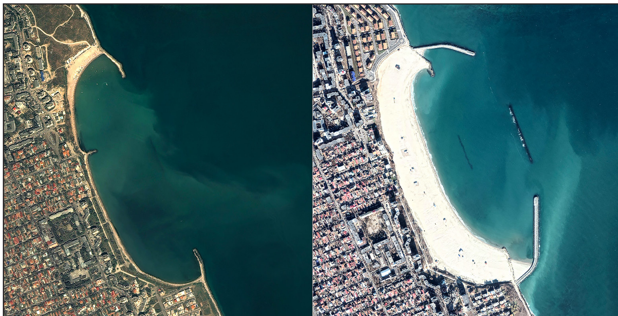
Fig. 1. Reyna study area before (left) and after (right) enlargement of the beach (Images: Google Earth – Maxar Technologies). The image to the right shows the new embankments together with the outer submerged spur dike. The inner spur dike was constructed previously. The former embankments, north and south of the bay were eliminated. The added sand widens the beach with approximately 120-130 m.
