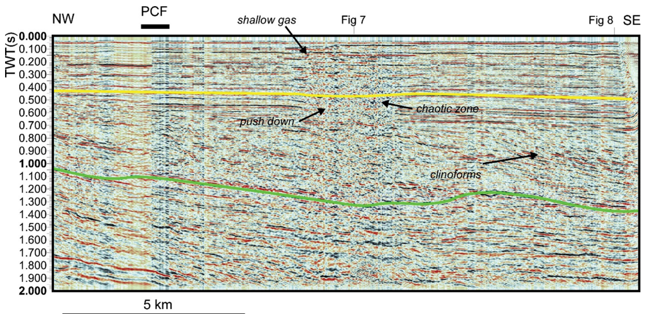
Fig. 6. Interpreted seismic line X2P2, over the southern border of Histria Basin. For localization see Fig. 1. We illustrate the zone where PCF should be located at deeper levels.
