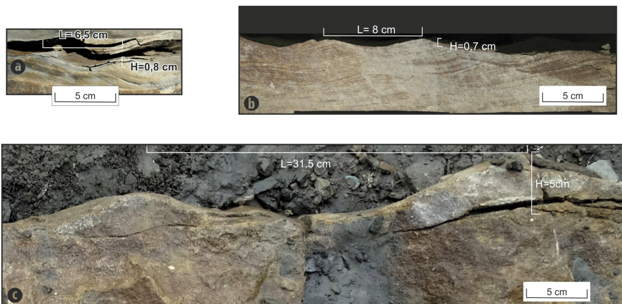
Fig. 24. Comparison between wave ripples from the sandstone-dominated Upper Meotian succession (a) and the oolith wave ripples (b). Râmnicul Sărat River, downstream from Jitia de Jos locality.
