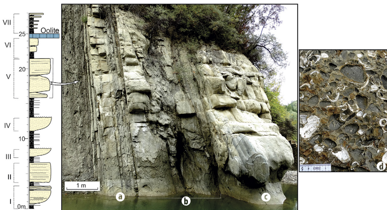
Fig. 8. Unit V, on top of the sandstone-dominated Upper Meotian sedimentary succession. (a), (b) and (c): Lithologic subunits. (d): Resedimented freshwater Unio shells associated with clay pebbles, occurring in subunit C.
