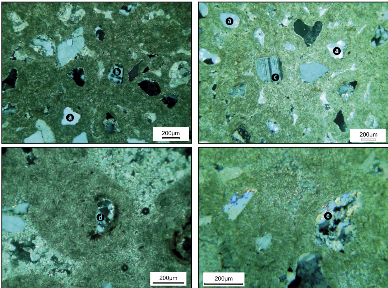
Fig. 21. Ooid nuclei represented by quartz (a), microcline feldspars (b), plagioclase feldspar (c), micro-quartzite (d) and micashist (e). Jitia de Jos oolitic limestone.
