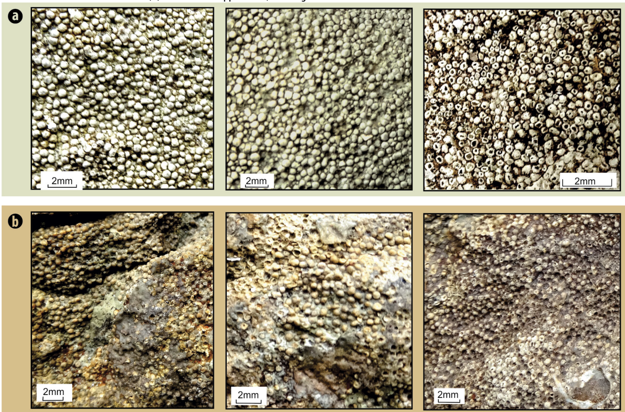
Fig. 14. Jitia de Jos oolit, on the upper surface of the bed (a) and in vertical sections (b).
