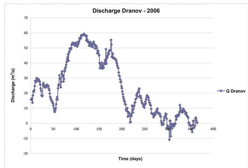
Fig. 3. Discharge on the Dranov channel
