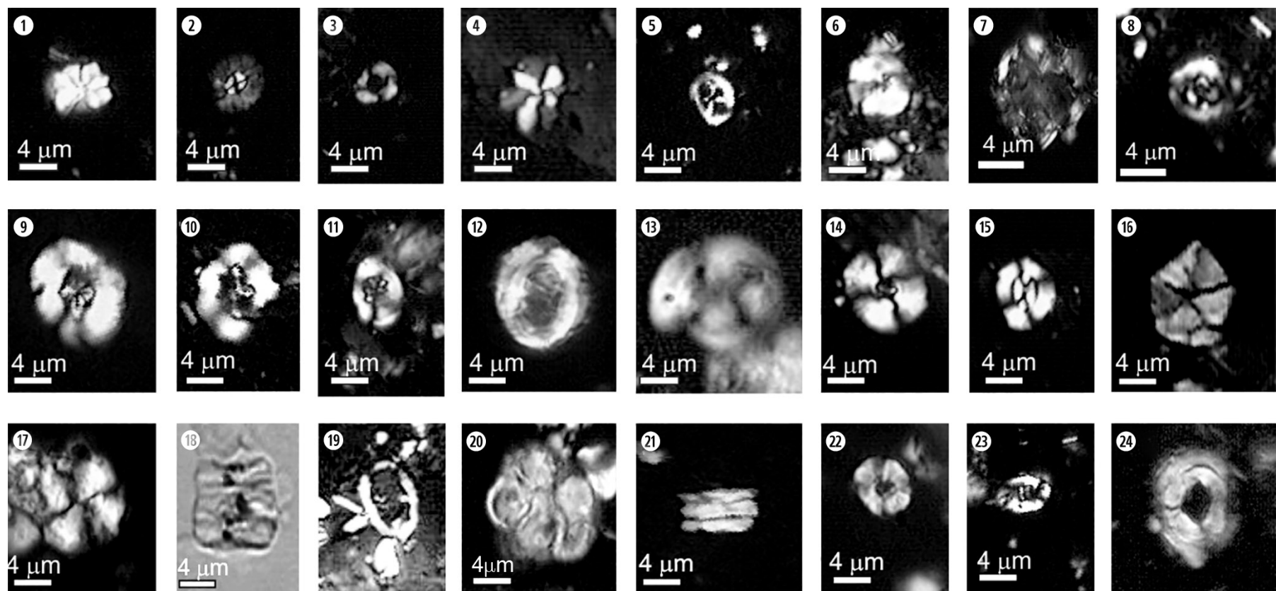
Fig. 6. Microphotographs of Valanginian calcareous nannofossils identified of studied Section 2 (Sinaia-Penny) taken under LM - light microscope, in N+ - crossed nicols, except 18 in NII – polarized lights; 1. Rucinolithus sp; Sample 35. 2. Biscutum constans (Górka, 1957) Black in Black and Barnes, 1959; Sample 11. 3. Diazomatolithus lehmanii Noël, 1965; Sample 11. 4. Rucinolithus pinnatus Bergen, 1994; Sample 21. 5. Staurolithites mutterlosei Crux, 1989; Sample 21. 6. Assipetra infracretacea (Thierstein, 1973) Roth, 1973; Sample 15. 7. Calicalathina oblongata (Worsley, 1971) Thierstein, 1971; Sample 15. 8. Helenea chias-tia Worsley, 1971; Sample 44. 9. Cruciellipsis cuvillierii (Manivit, 1966) Thierstein, 1971; Sample 28. 10. Cretarhabdus conicus Bramlette & Martini, 1964; Sample 28. 11. Retecapsa angustiforata Black, 1971; Sample 40. 12. Tubodiscus jurapelagicus (Worsley, 1971) Roth, 1973; Sample 2. 13. Haqius circumradiatus (Stover, 1966) Roth, 1978; Sample 40. 14. Watznaueria britannica (Stradner, 1963) Reinhardt, 1964; Sample 29. 15. Watznaueria barnesiae (Black in Black & Barnes, 1959) Perch-Nielsen, 1968; Sample 29. 16. Micrantholithus hoschulzii (Reinhardt, 1966) Thierstein, 1971; Sample 29. 17. Cyclagelosphaera brezae Applegate & Bergen, 1988; Sample 40. 18. Nannoconus kamptneri Brönnimann, 1955; Sample 17. 19. Diloma galiciense Bergen, 1994; Sample 43. 20. Braarudosphaera primula Black, 1973; Sample 18. 21. Conusphaera mex-icana subsp. mexicana Trejo, 1969; Sample 17. 22. Tegulalithus septentrionalis (Stradner, 1963) Crux, 1986; Sample 45. 23. Eiffelithus windii Applegate & Bergen, 1988; Sample; 24. Tubodiscus verena Thierstein, 1973; Sample 2.
