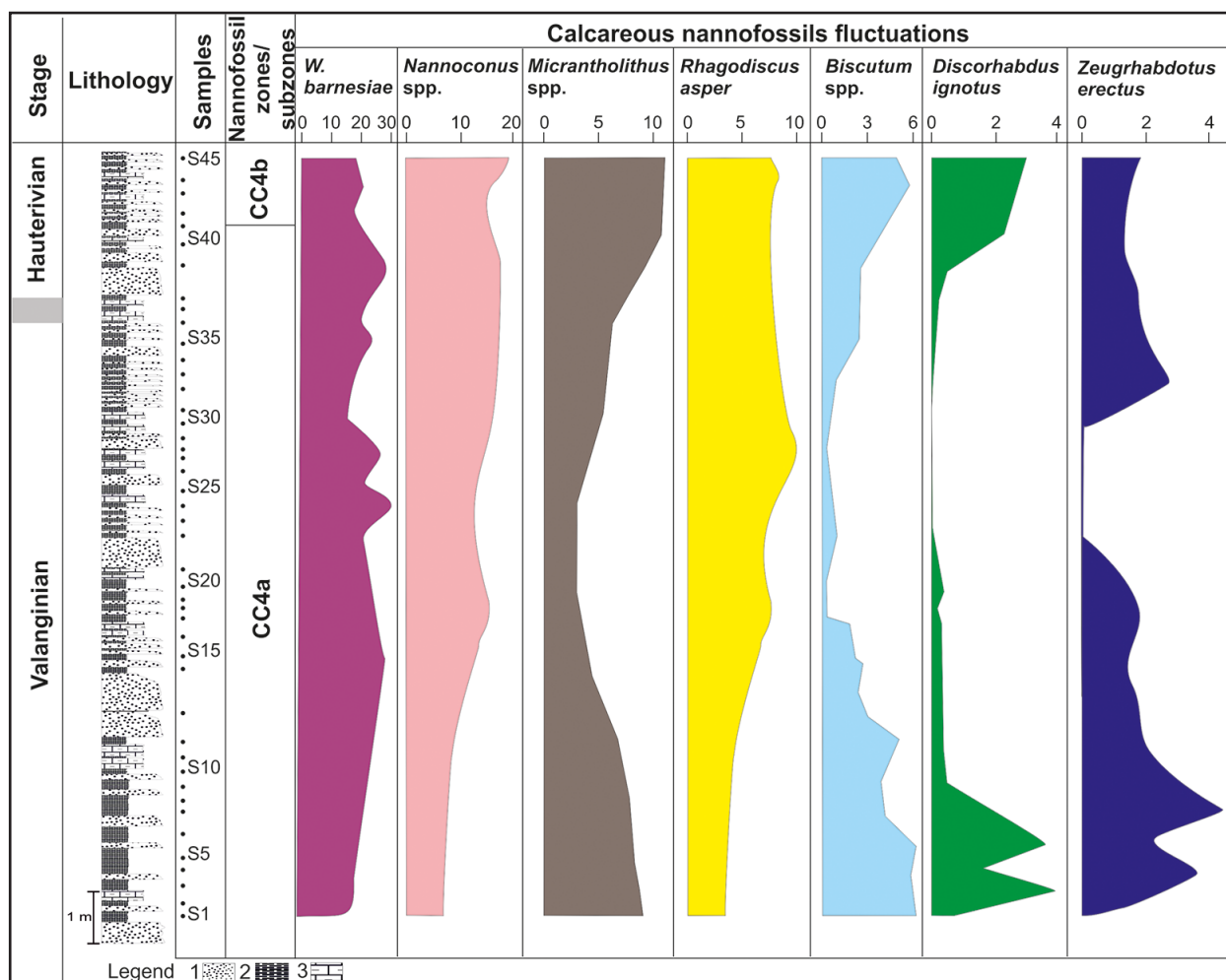
Fig. 7. Calcareous nannofossil fluctuation in the studied Section 2 (Sinaia-Penny), southern end of the Eastern Carpathians. Legend: 1 - sandstones; 2 - dark grey and black shales; 3 - sandstones.
