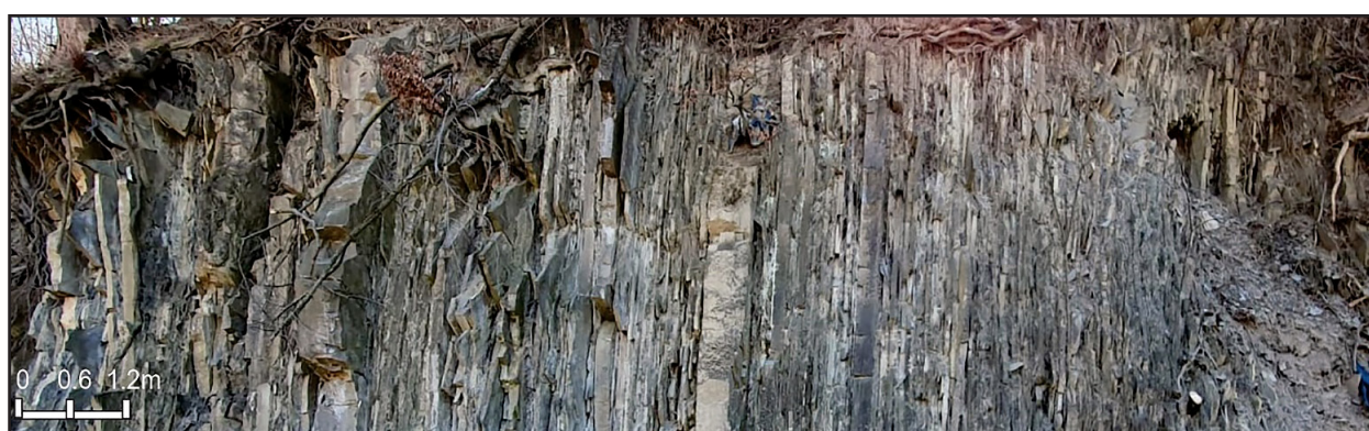
Fig. 5. The investigated succession of the Sinaia Formation Sinaia-Penny (N exit of the Sinaia town).
