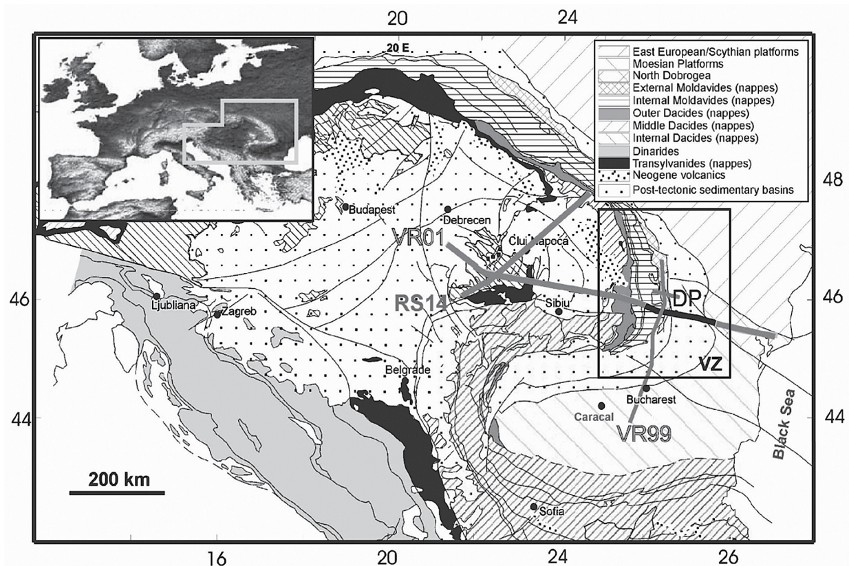
Fig. 1. Tectonic map of the Carpathians/Dinarides/Pannonian Basin system in southeastern Europe showing setting of the deep reflection (DP) and deep refraction (VR99, VR01, RS14) seismic profiles; VZ – Vrancea earthquake zone (modified after Sandulescu, 1984).
